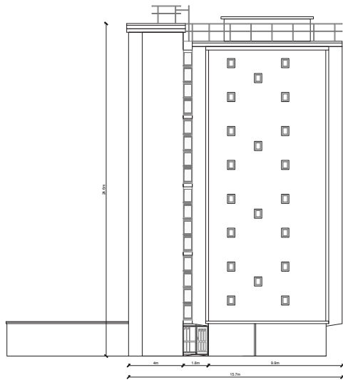
Residential Flats - North Elevation
